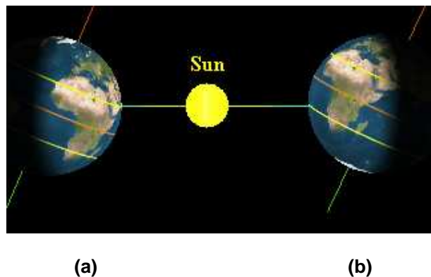
Figure 1: Austral seasons. (a) Summer [winter] in northern [southern] hemisphere. (b) Summer [winter] in southern [northern] hemisphere
