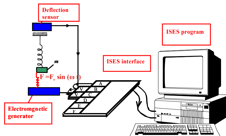
Figure 1 The schematic representation of the remote experiment Driven oscillator with mass and spring using the system ISES. The oscillator consists of the spring and the weight, the external force is exerted by the electromagnetic generator with the variable frequency, all controlled by ISES, the instantaneous deflection is detected by the deflection sensor.
