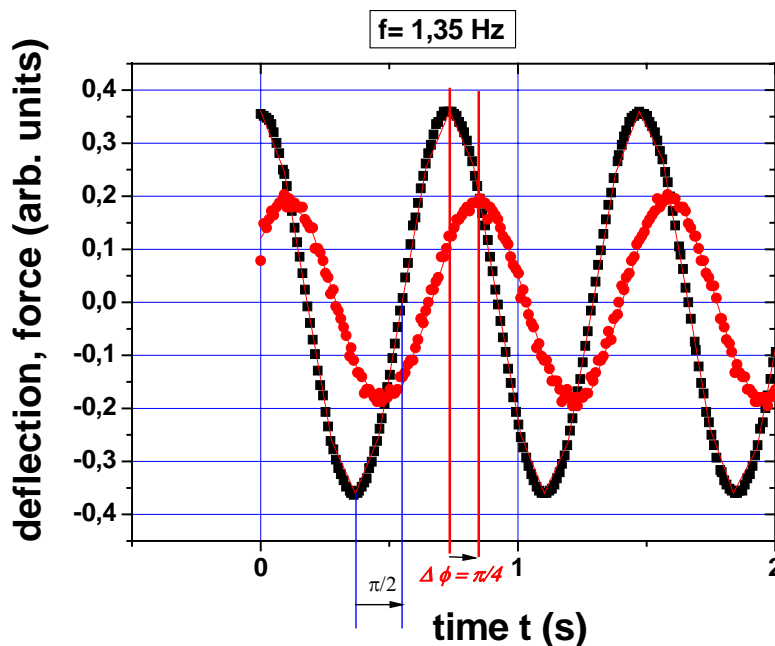
Figure 3 Time dependence of the external force (black points) and instantaneous deflection (red points) of the spring and mass mechanical oscillator measured by ISES system for the external force with below resonance frequency f=1,35 Hz, the phase shift \Delta\Phi = \pi/4 is also depicted. The red lines are the least squares fit.
