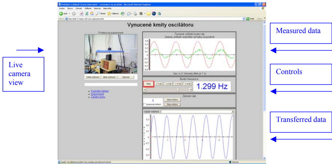
Figure 2 The web page of the real remote experiment Driven oscillator with frequency controls, live web camera view and graph of the measured data (upper plate: red - driving force, green - instantaneous deflection, below: transferred data – here the driving force, the second part of the transferred data is hidden).
