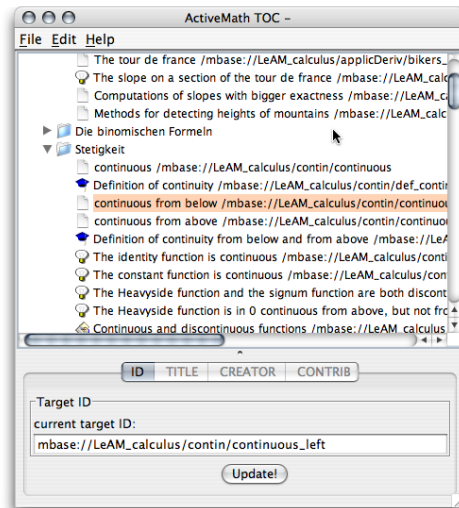
FIGURE 2: The table-of-contents editor.
