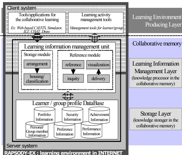
Figure 3 : The Mechanism Scheme of the Knowledge Marketplace (i.e. REX)
