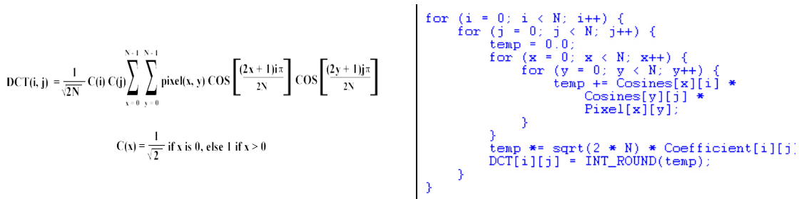
FIGURE 1: DCT transformation for a NxN pixels image and corresponding C code.
