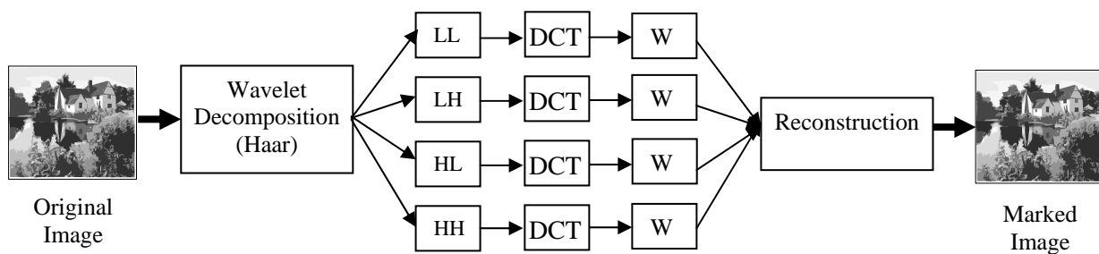
FIGURE 2: Subband DCT watermarking process
